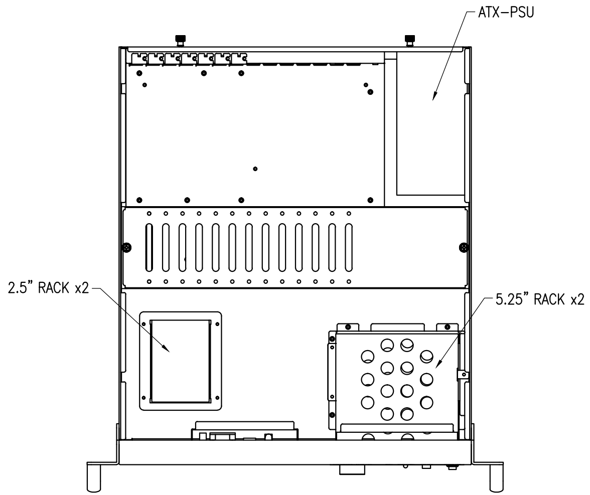
TOP-IN SIDE VIEW
